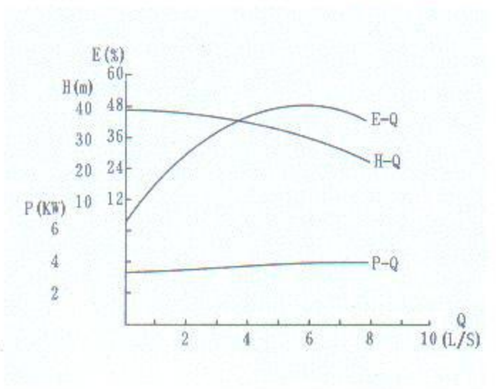
ZW50-20-35
